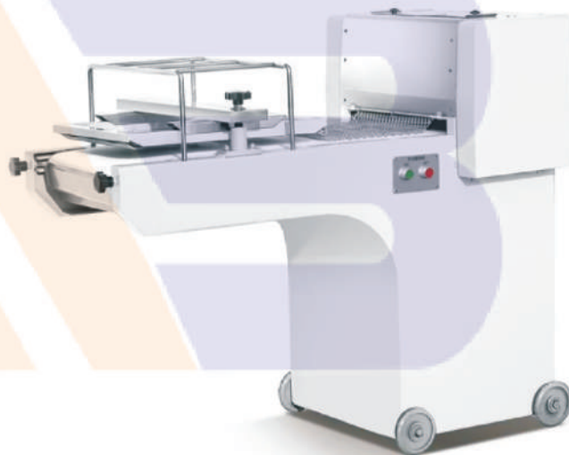
Dough Moulder Size : 58X134X110 inches Capacity : 1000/3000 pcs/Hr Dough Weight : 50 - 120gm
